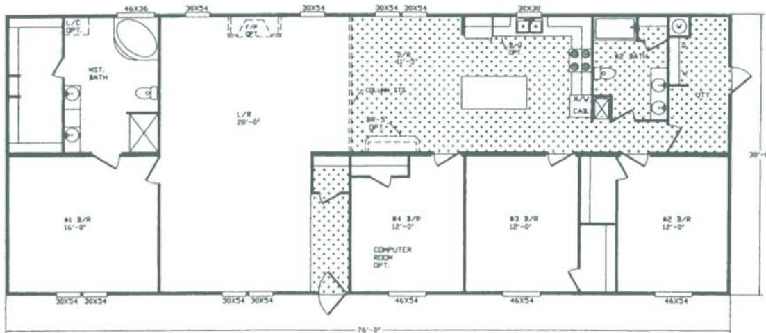
MODEL 3007 80 x 32 4 Bedroom 3 Bath 2280 Sq. Ft.
